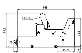
OPT printhead – Top connector
