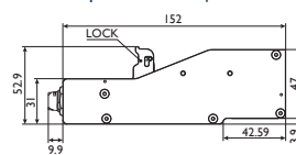
Standard printhead – Top connector
